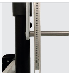
Easy to use, tapered component reel holder
